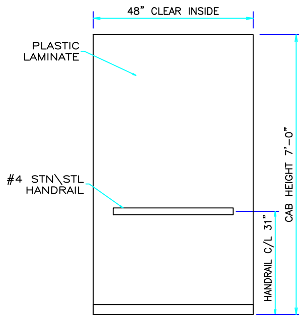
ELEVATION C
