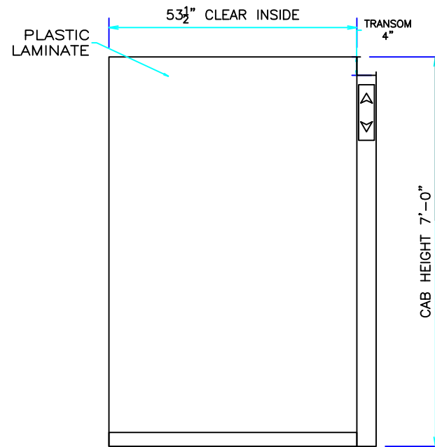
ELEVATION D
