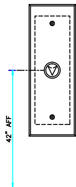
TERMINAL HALL STATION FINISH: #4 STN\STL BOX DEPTH 3 1/2" QUANTITY: 1
